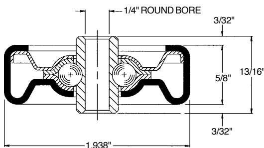
Part No. 102144
